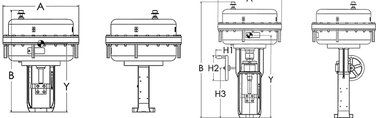
23L Shown without optional Handwheel
